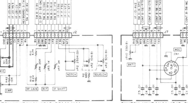
CONTROL UNIT (X53-1450-00) (B/2)
