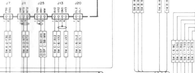
FILTER UNIT (X51-1340-00)
