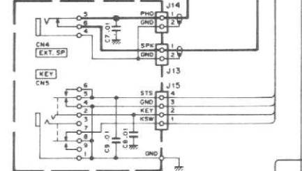
SWITCH UNIT (X41-1610-00) (G/14)
