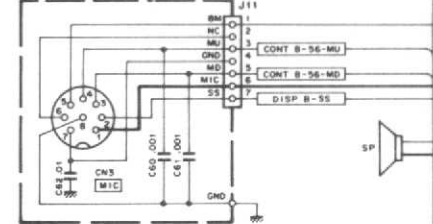
SWITCH UNIT (X41-1610-00) (D/14)
