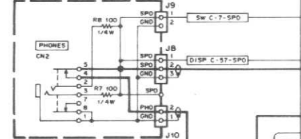
SWITCH UNIT (X41-1610-00) (G/14)
