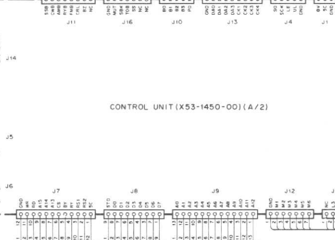
CONTROL UNIT (X53-1450-00) (A/2)
