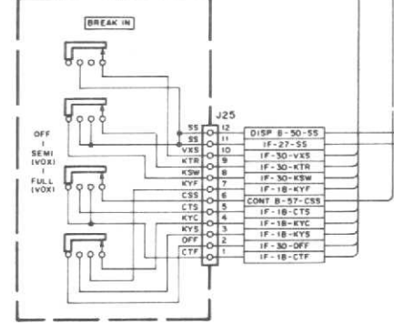
SWITCH UNIT (X41-1610-00) (L/14)
