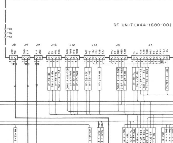
RF UNIT (X44-1680-00)
